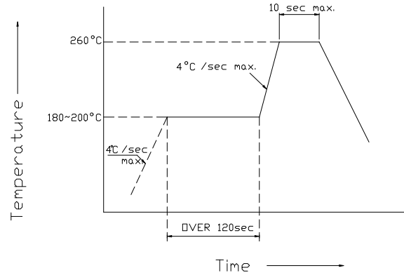
Lead-Free Solder 无铅回焊
