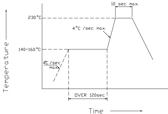
Lead Solder 有铅回焊
